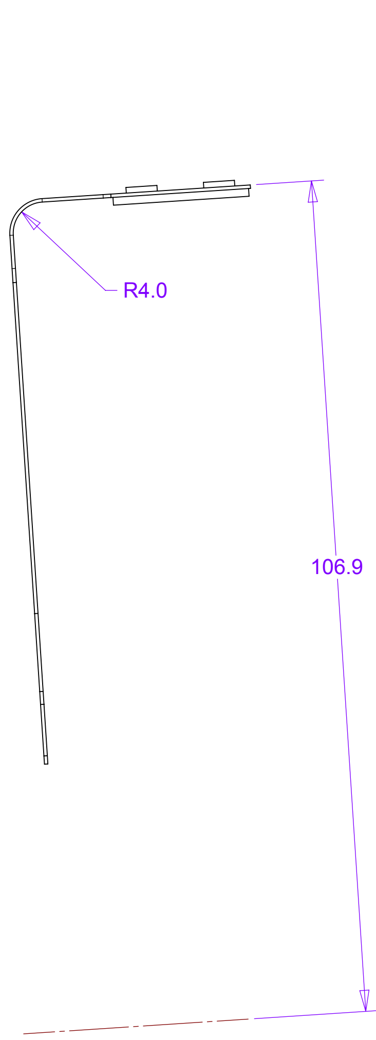
VIEW C-C
